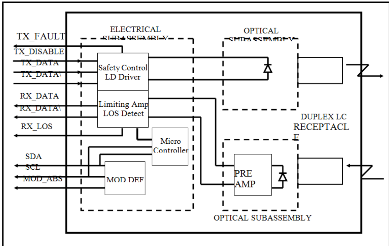
Block Diagram of Transceiver
